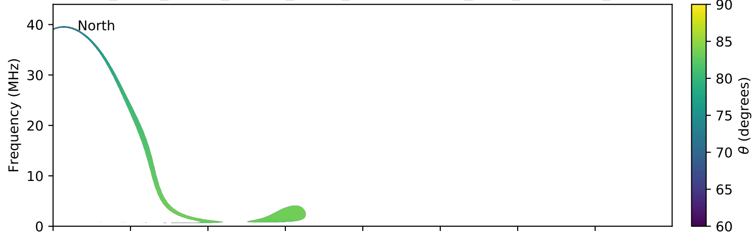
expres_earth_jupiter_europa_jrm09_lossc-wid1deg_3kev_20070627_v01.cdf
