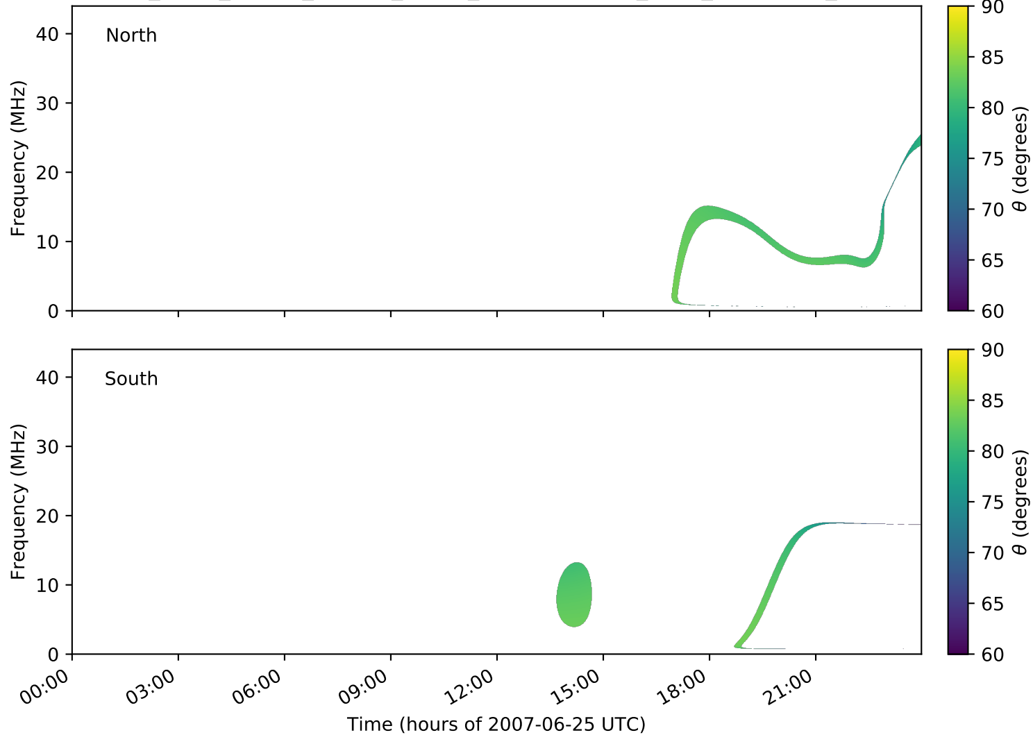
expres_earth_jupiter_europa_jrm09_lossc-wid1deg_3kev_20070625_v01.cdf
