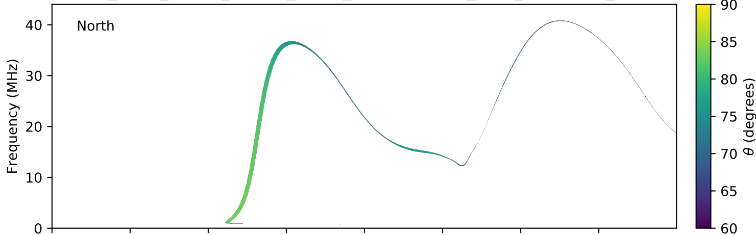
expres_earth_jupiter_europa_jrm09_lossc-wid1deg_3kev_20070622_v01.cdf
