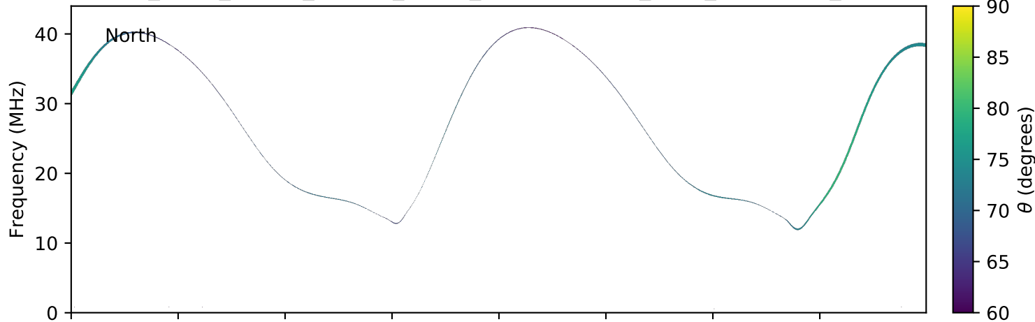
expres_earth_jupiter_europa_jrm09_lossc-wid1deg_3kev_20070619_v01.cdf
