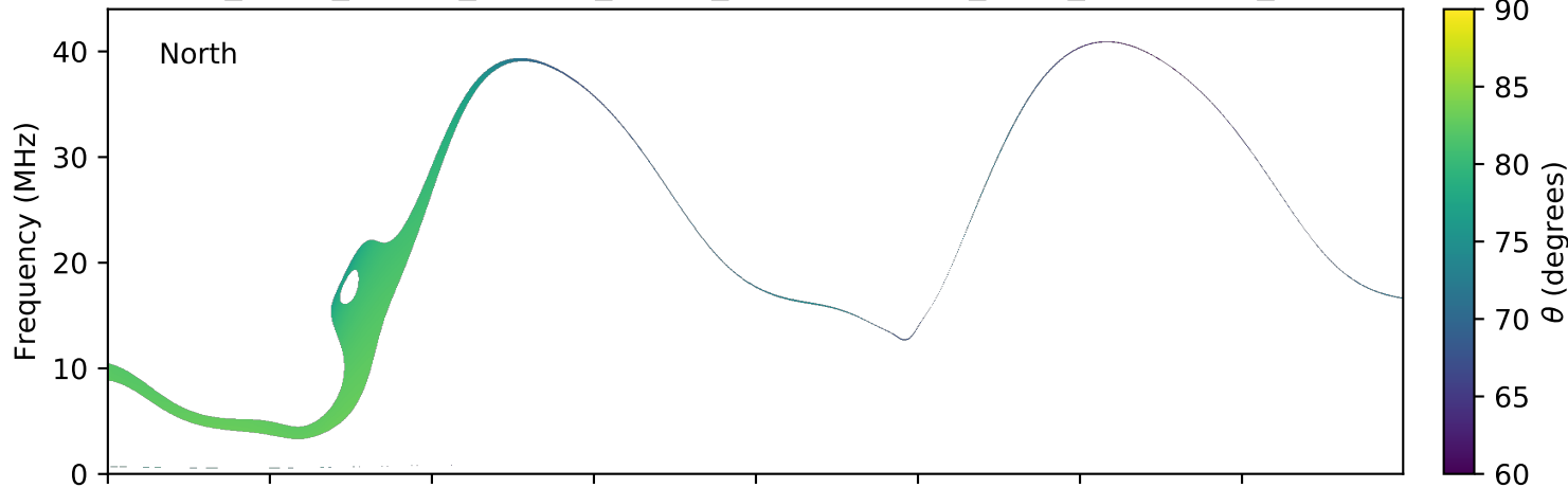
expres_earth_jupiter_europa_jrm09_lossc-wid1deg_3kev_20070608_v01.cdf
