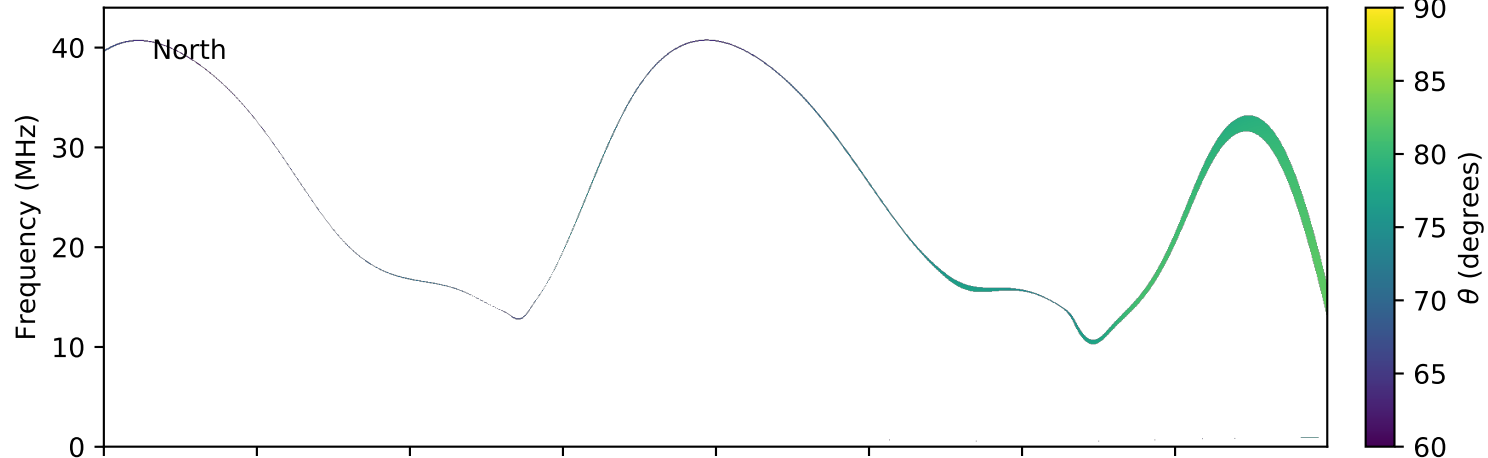
expres_earth_jupiter_europa_jrm09_lossc-wid1deg_3kev_20070605_v01.cdf
