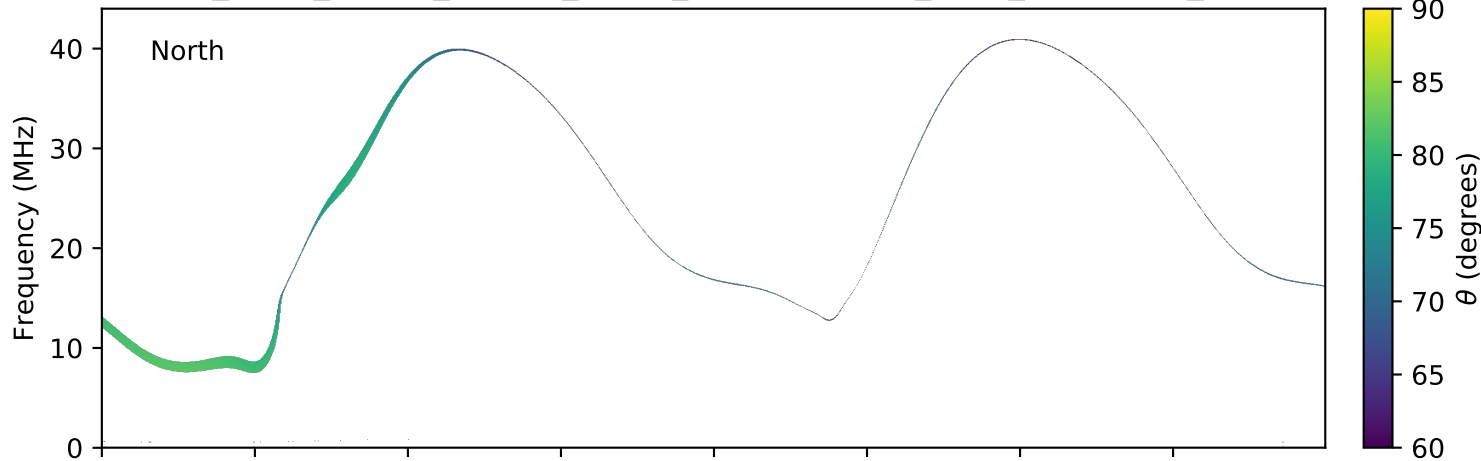
expres_earth_jupiter_europa_jrm09_lossc-wid1deg_3kev_20070601_v01.cdf
