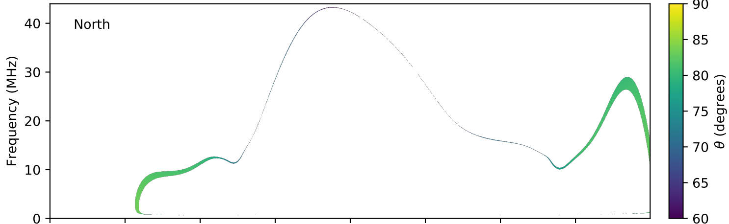
expres_earth_jupiter_io_jrm09_lossc-wid1deg_3kev_20070531_v01.cdf
