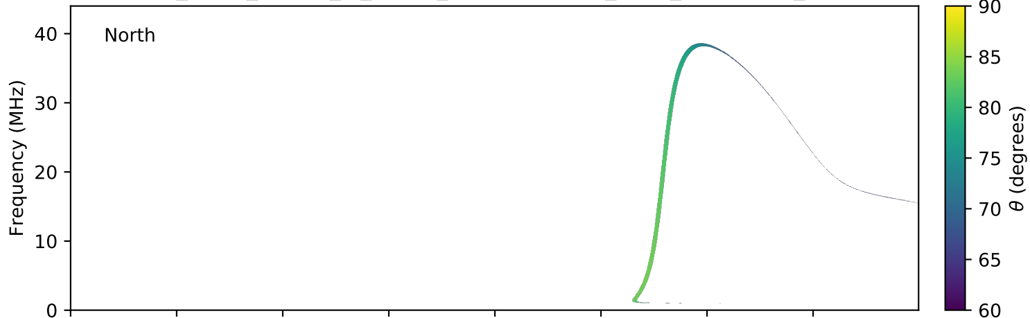
expres_earth_jupiter_io_jrm09_lossc-wid1deg_3kev_20070527_v01.cdf
