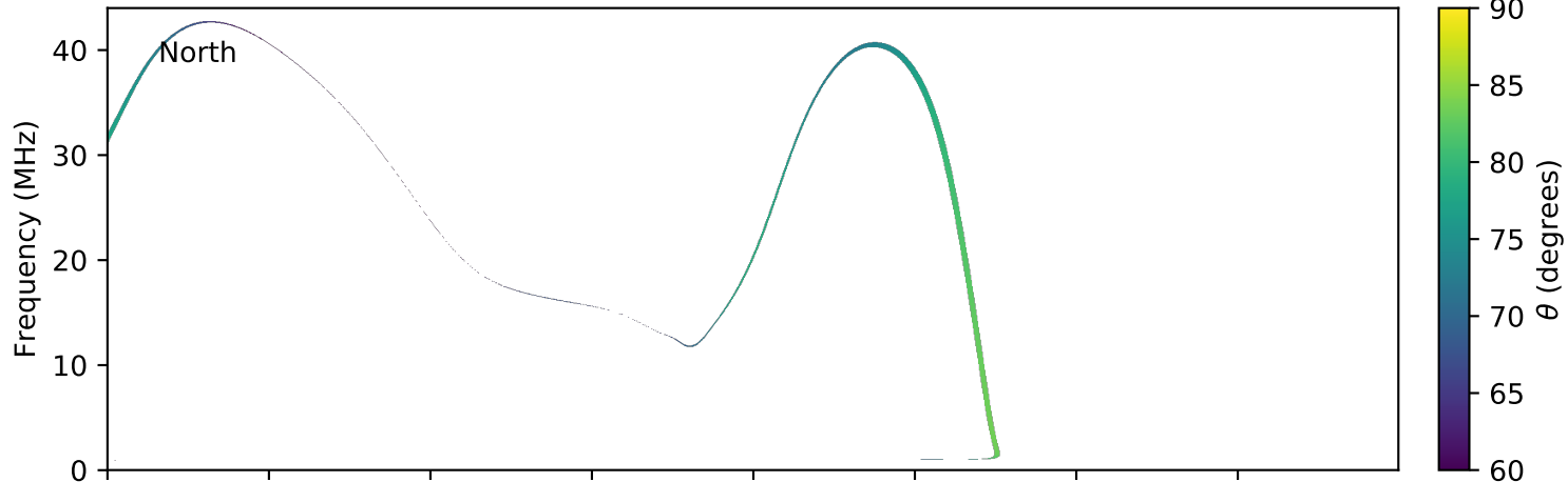
expres_earth_jupiter_io_jrm09_lossc-wid1deg_3kev_20070526_v01.cdf
