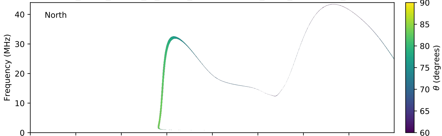
expres_earth_jupiter_io_jrm09_lossc-wid1deg_3kev_20070522_v01.cdf
