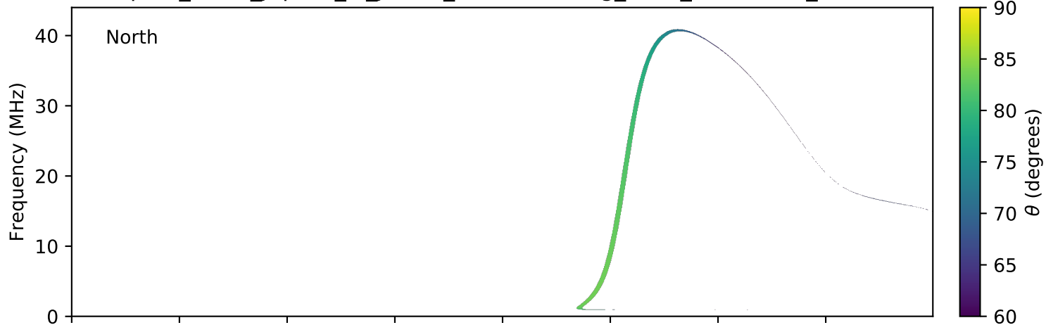
expres_earth_jupiter_io_jrm09_lossc-wid1deg_3kev_20070520_v01.cdf
