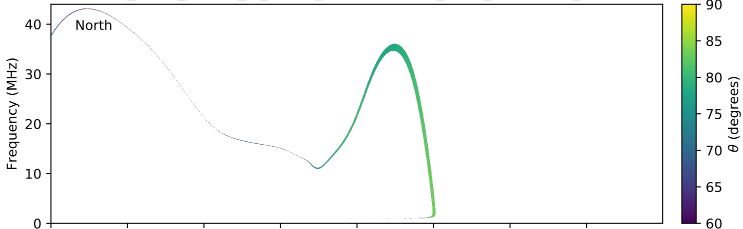
expres_earth_jupiter_io_jrm09_lossc-wid1deg_3kev_20070519_v01.cdf
