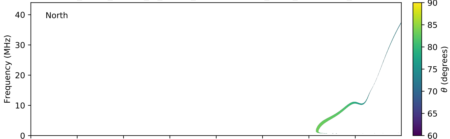
expres_earth_jupiter_io_jrm09_lossc-wid1deg_3kev_20070518_v01.cdf
