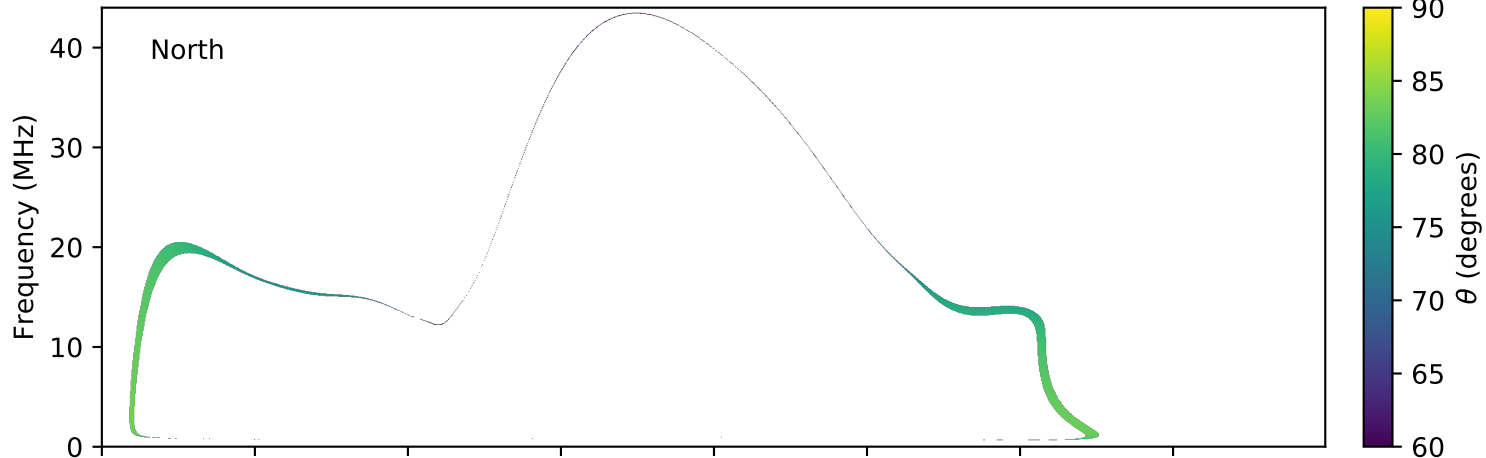
expres_earth_jupiter_io_jrm09_lossc-wid1deg_3kev_20070517_v01.cdf
