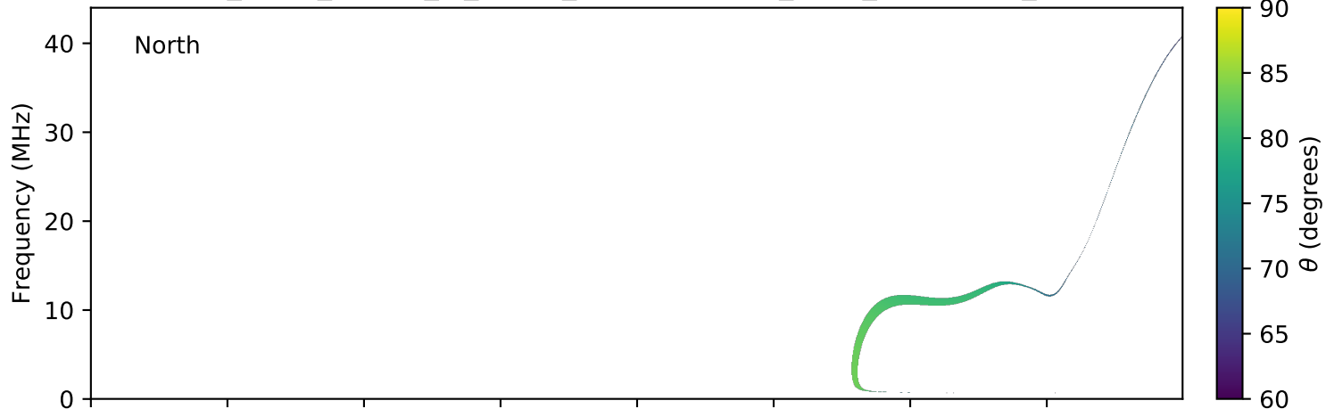
expres_earth_jupiter_io_jrm09_lossc-wid1deg_3kev_20070511_v01.cdf
