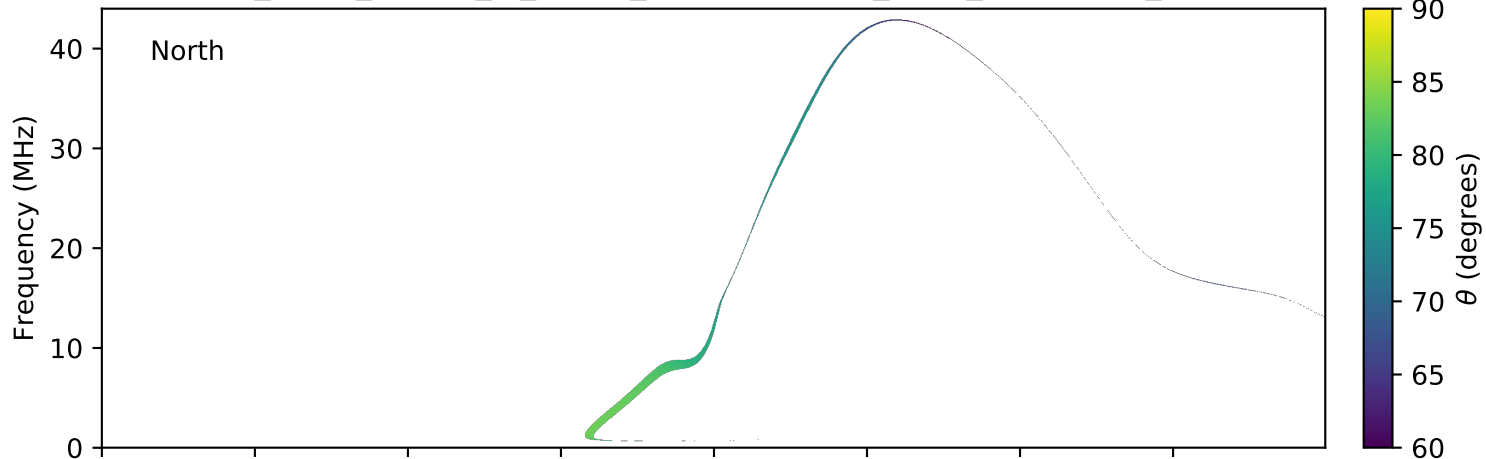
expres_earth_jupiter_io_jrm09_lossc-wid1deg_3kev_20070506_v01.cdf
