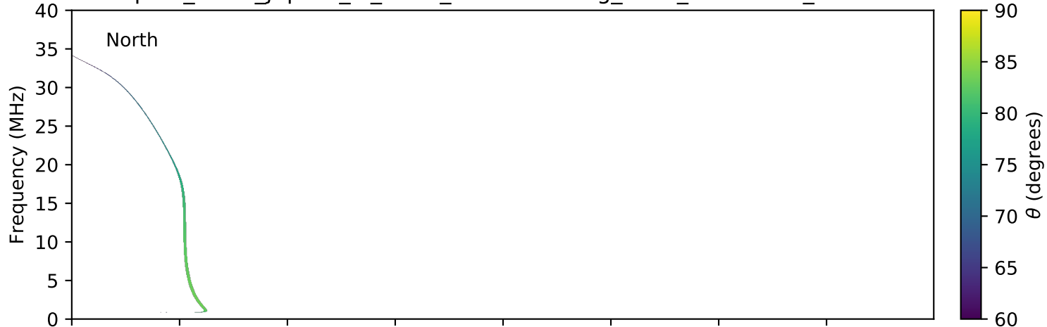
expres_earth_jupiter_io_isaac_lossc-wid1deg_3kev_20070530_v01.cdf
