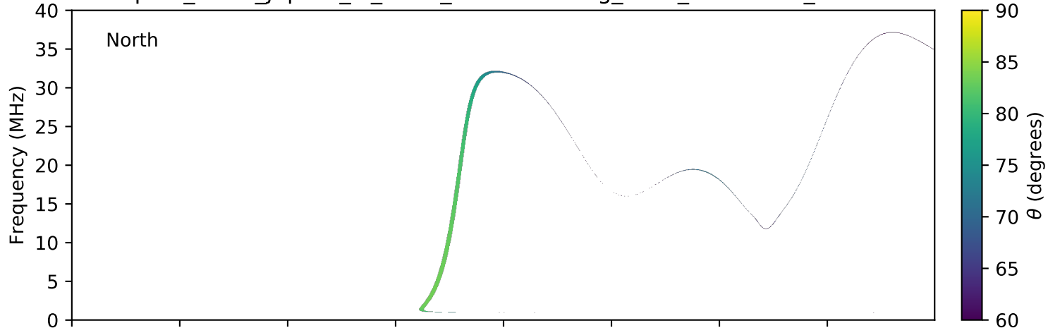
expres_earth_jupiter_io_isaac_lossc-wid1deg_3kev_20070529_v01.cdf
