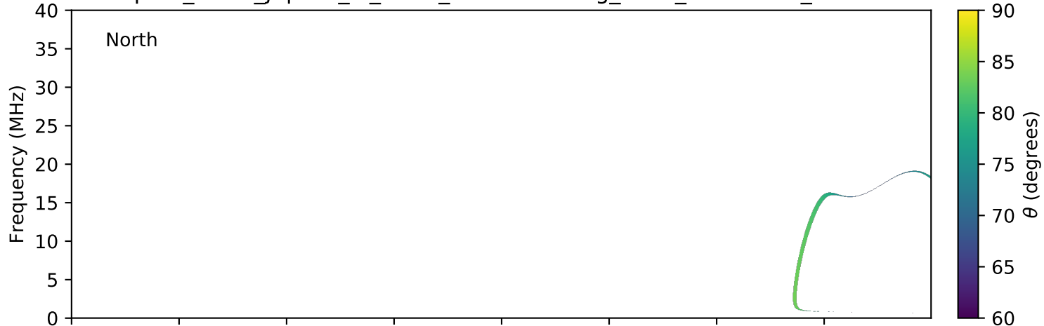
expres_earth_jupiter_io_isaac_lossc-wid1deg_3kev_20070525_v01.cdf
