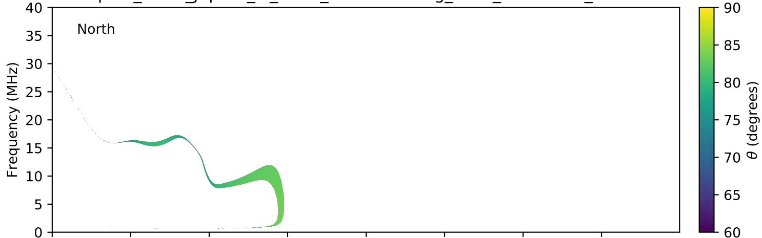
expres_earth_jupiter_io_isaac_lossc-wid1deg_3kev_20070521_v01.cdf
