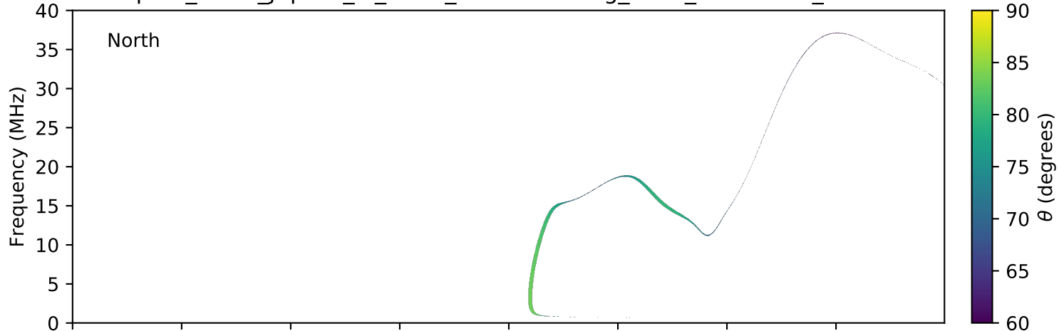
expres_earth_jupiter_io_isaac_lossc-wid1deg_3kev_20070520_v01.cdf
