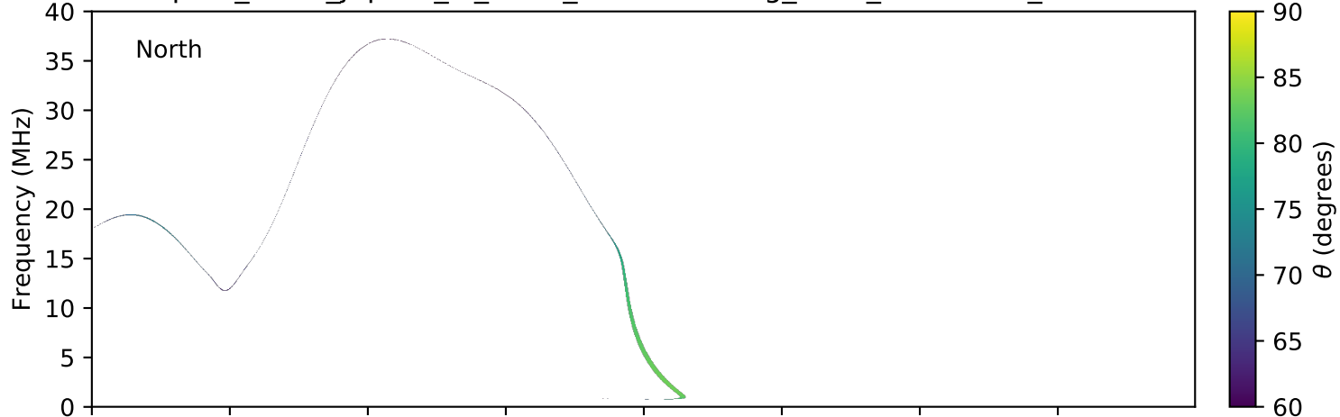
expres_earth_jupiter_io_isaac_lossc-wid1deg_3kev_20070519_v01.cdf
