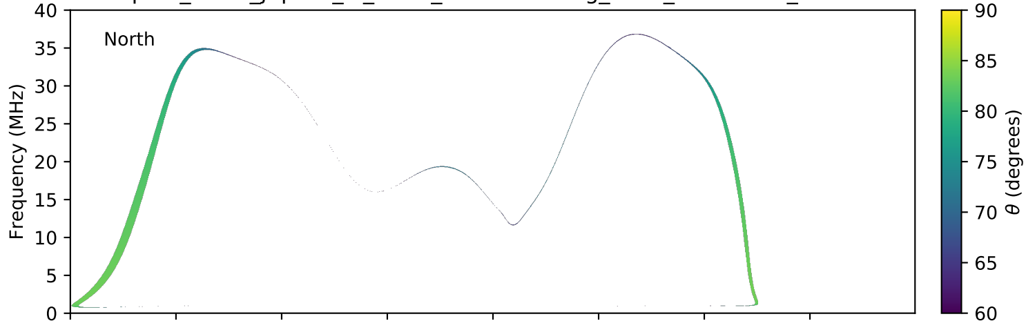
expres_earth_jupiter_io_isaac_lossc-wid1deg_3kev_20070517_v01.cdf
