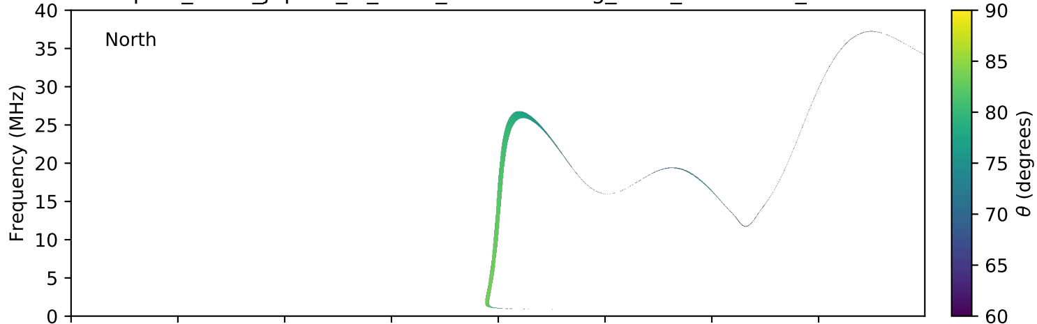
expres_earth_jupiter_io_isaac_lossc-wid1deg_3kev_20070513_v01.cdf
