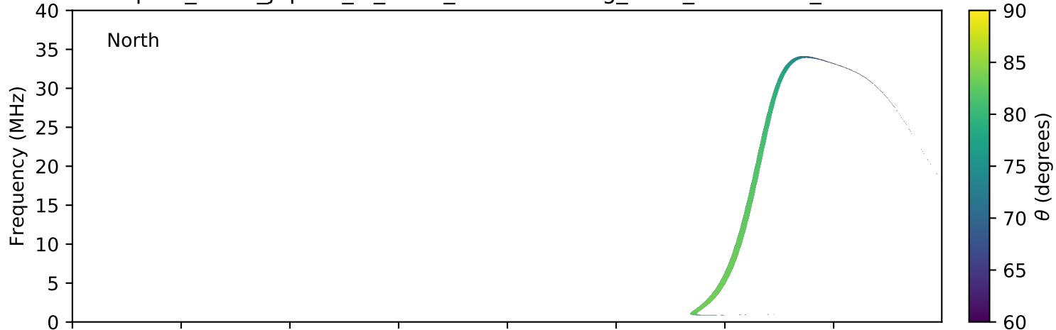
expres_earth_jupiter_io_isaac_lossc-wid1deg_3kev_20070511_v01.cdf
