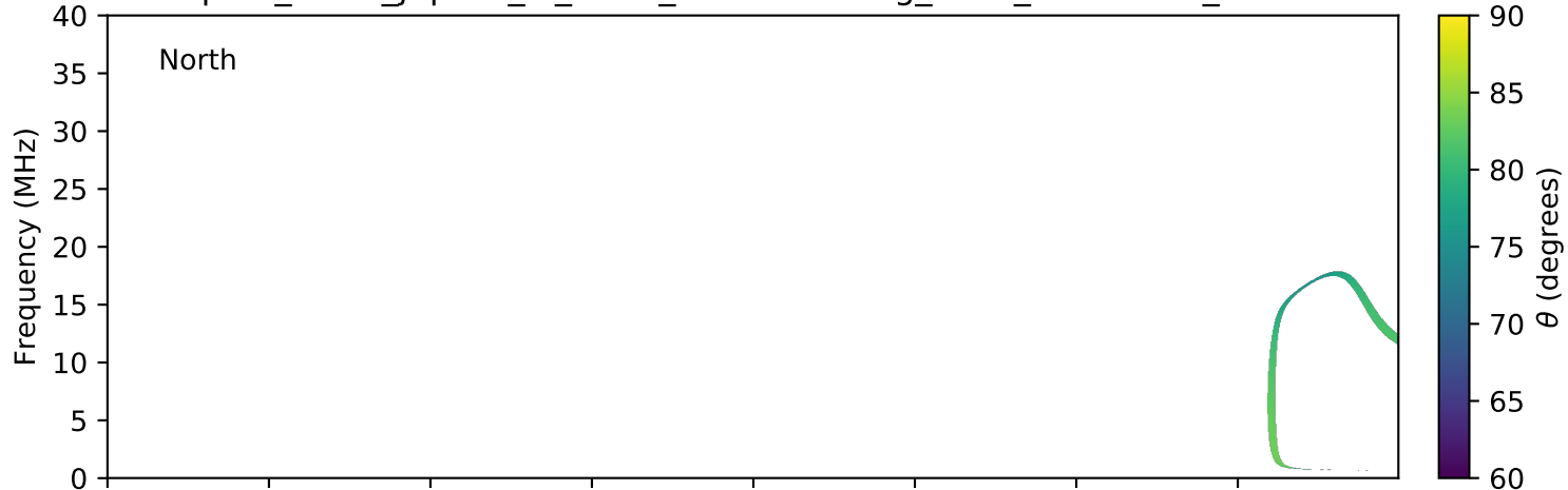
expres_earth_jupiter_io_isaac_lossc-wid1deg_3kev_20070509_v01.cdf
