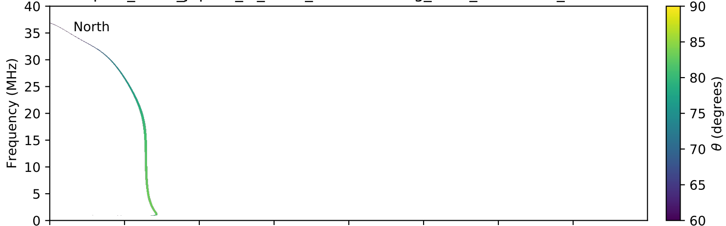
expres_earth_jupiter_io_isaac_lossc-wid1deg_3kev_20070507_v01.cdf
