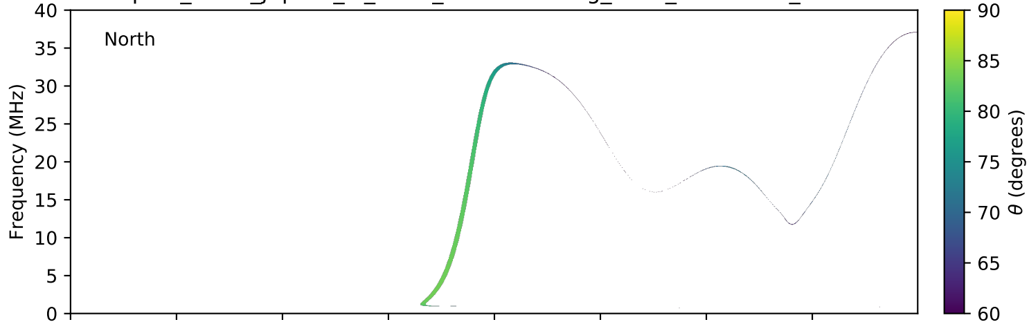
expres_earth_jupiter_io_isaac_lossc-wid1deg_3kev_20070506_v01.cdf
