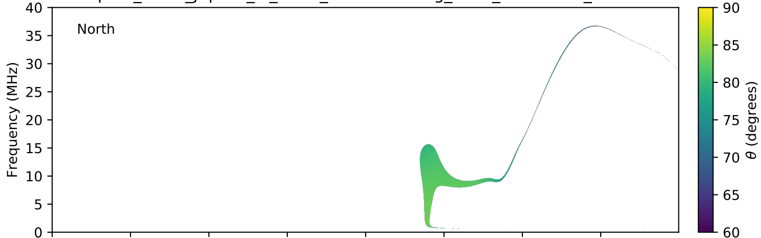
expres_earth_jupiter_io_isaac_lossc-wid1deg_3kev_20070504_v01.cdf
