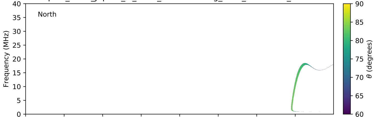
expres_earth_jupiter_io_isaac_lossc-wid1deg_3kev_20070502_v01.cdf
