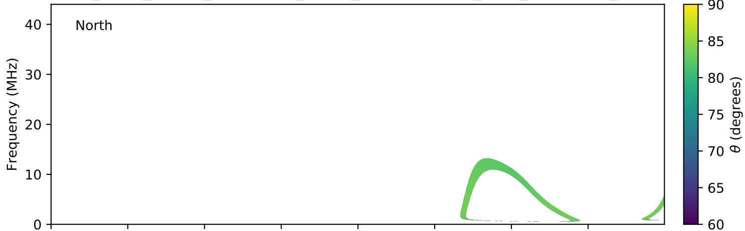
expres_earth_jupiter_ganymede_jrm09_lossc-wid1deg_3kev_20070506_v01.cdf
