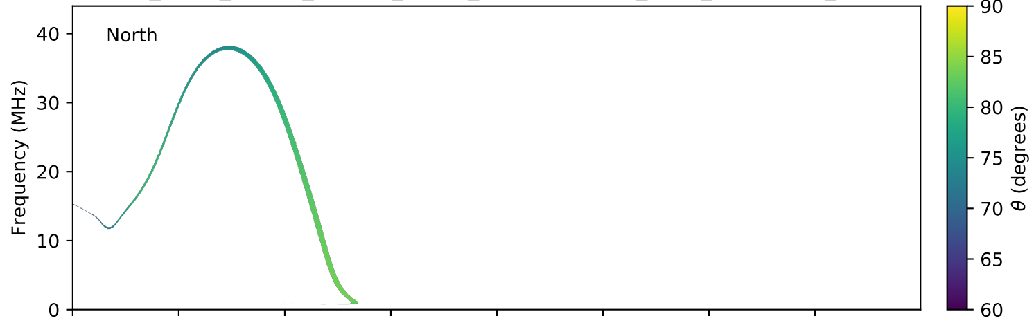
expres_earth_jupiter_europa_jrm09_lossc-wid1deg_3kev_20070526_v01.cdf
