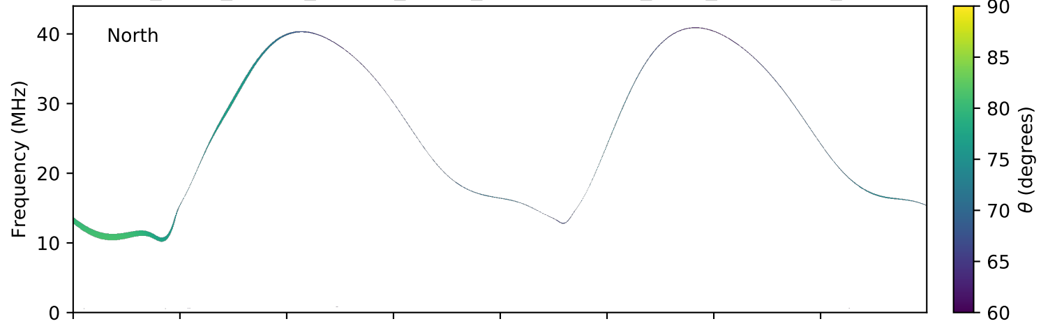
expres_earth_jupiter_europa_jrm09_lossc-wid1deg_3kev_20070525_v01.cdf
