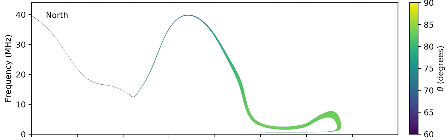
expres_earth_jupiter_europa_jrm09_lossc-wid1deg_3kev_20070515_v01.cdf
