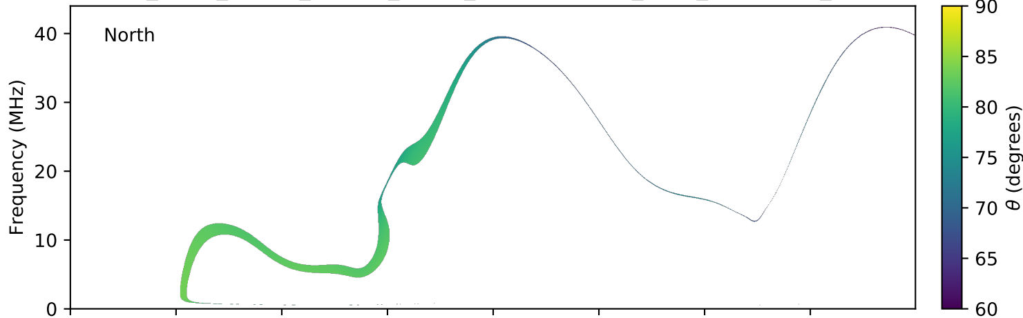
expres_earth_jupiter_europa_jrm09_lossc-wid1deg_3kev_20070514_v01.cdf
