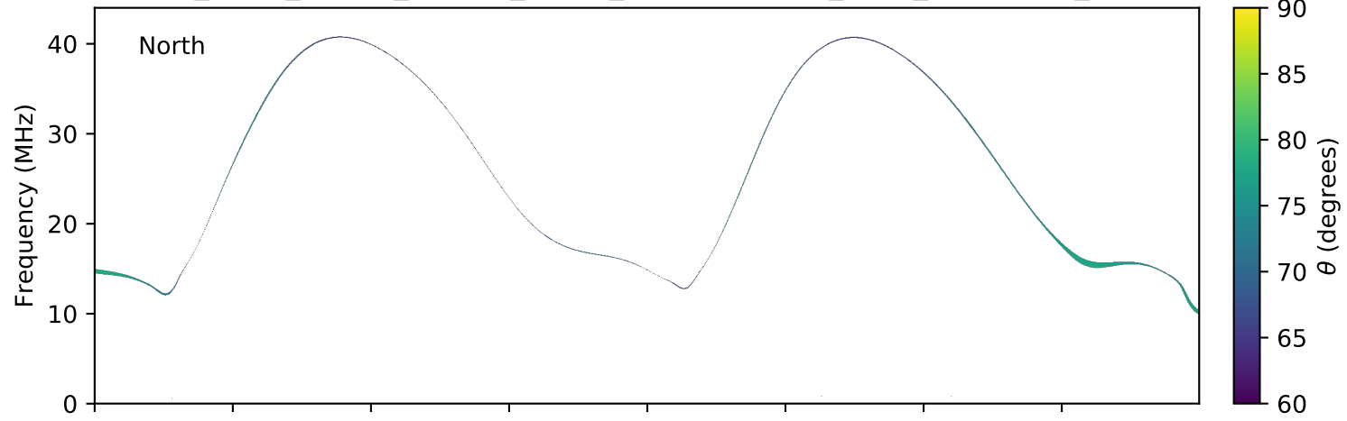
expres_earth_jupiter_europa_jrm09_lossc-wid1deg_3kev_20070511_v01.cdf
