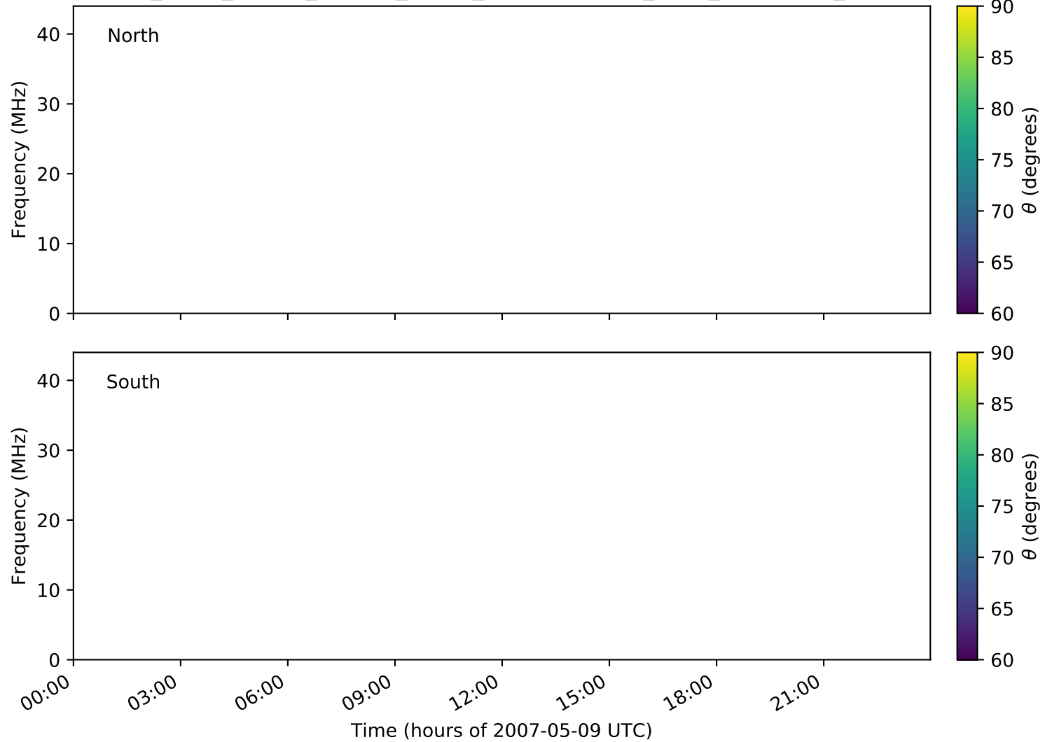
expres_earth_jupiter_europa_jrm09_lossc-wid1deg_3kev_20070509_v01.cdf
