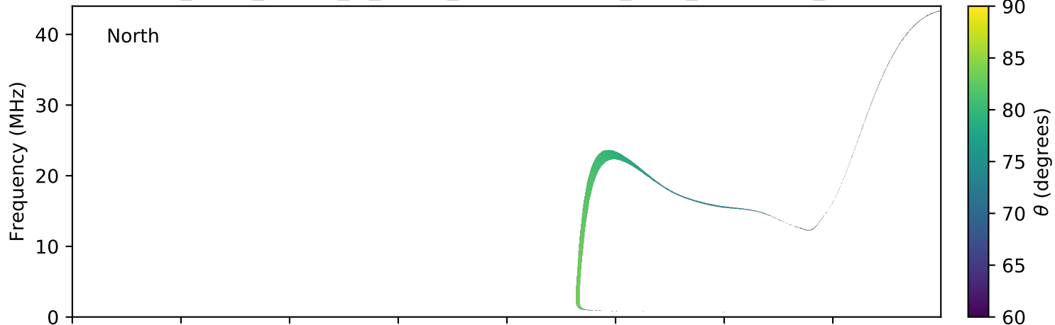
expres_earth_jupiter_io_jrm09_lossc-wid1deg_3kev_20070427_v01.cdf
