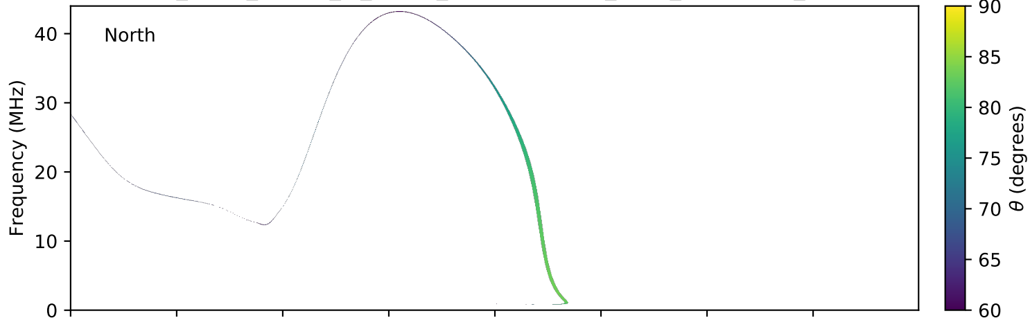
expres_earth_jupiter_io_jrm09_lossc-wid1deg_3kev_20070426_v01.cdf
