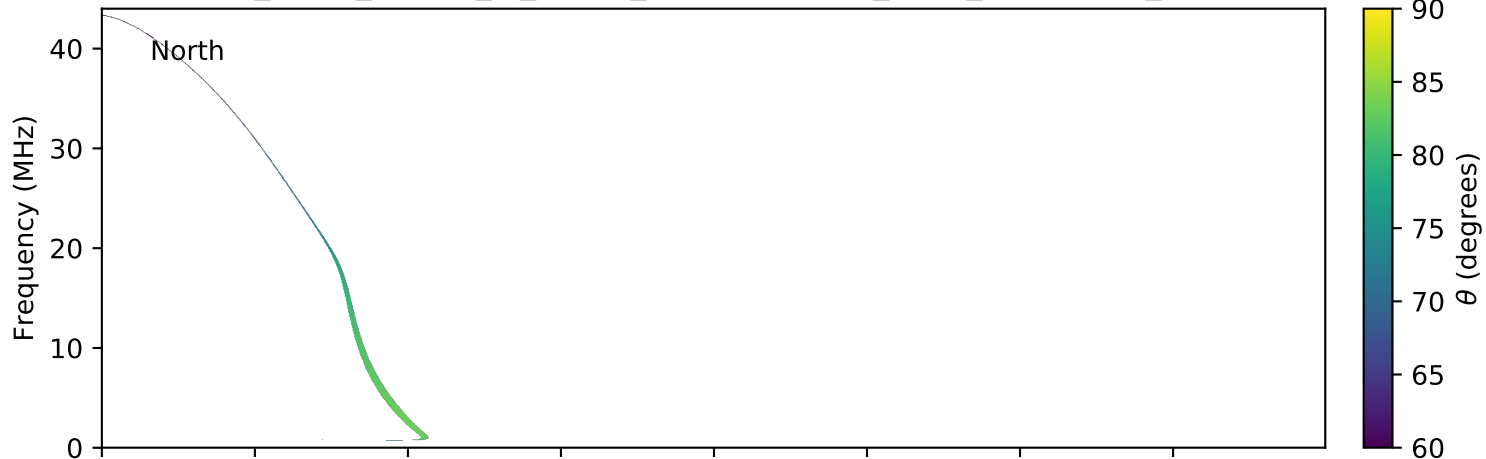
expres_earth_jupiter_io_jrm09_lossc-wid1deg_3kev_20070421_v01.cdf
