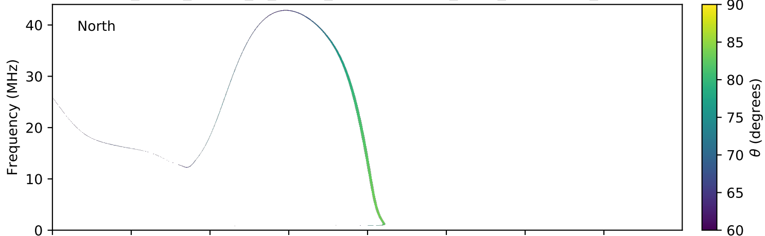
expres_earth_jupiter_io_jrm09_lossc-wid1deg_3kev_20070419_v01.cdf
