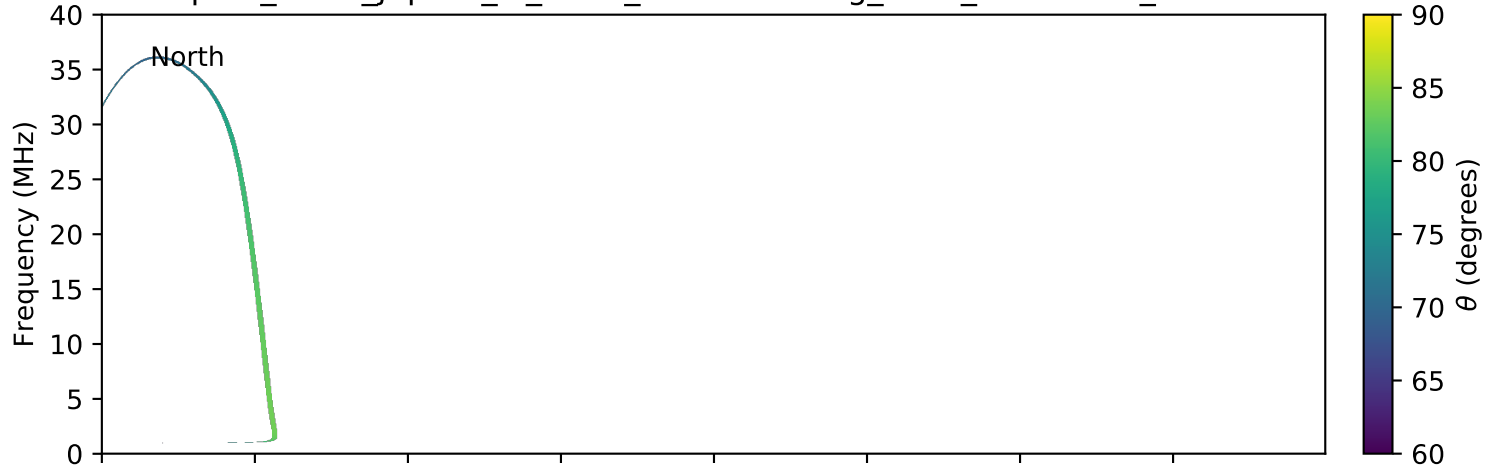
expres_earth_jupiter_io_isaac_lossc-wid1deg_3kev_20070430_v01.cdf
