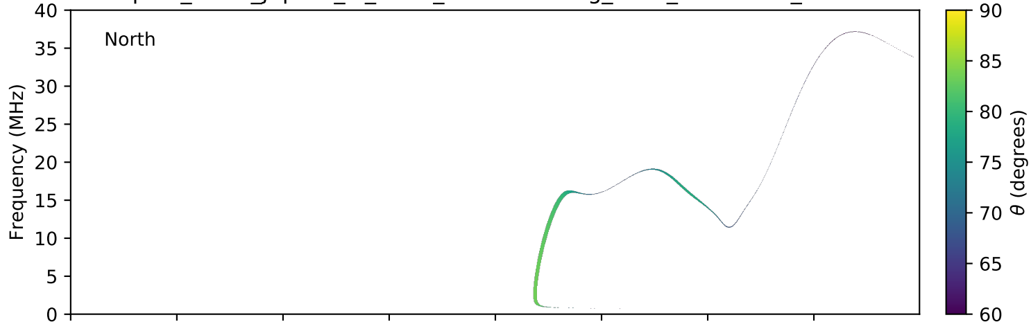
expres_earth_jupiter_io_isaac_lossc-wid1deg_3kev_20070427_v01.cdf
