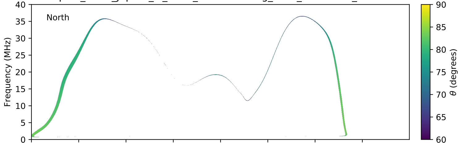
expres_earth_jupiter_io_isaac_lossc-wid1deg_3kev_20070424_v01.cdf
