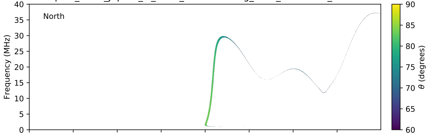
expres_earth_jupiter_io_isaac_lossc-wid1deg_3kev_20070420_v01.cdf
