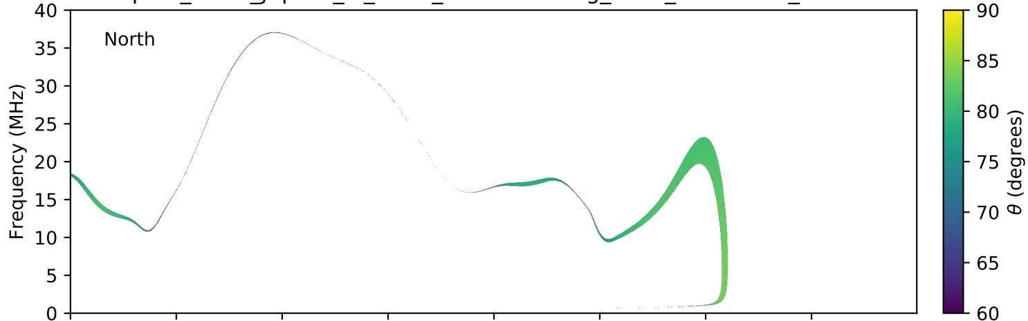
expres_earth_jupiter_io_isaac_lossc-wid1deg_3kev_20070417_v01.cdf
