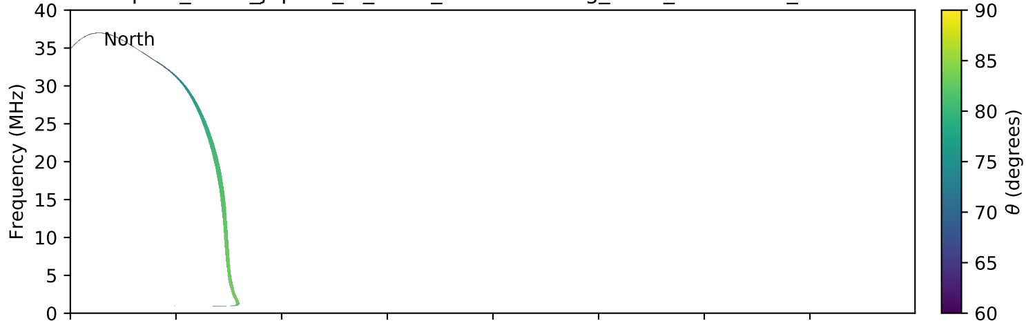
expres_earth_jupiter_io_isaac_lossc-wid1deg_3kev_20070414_v01.cdf
