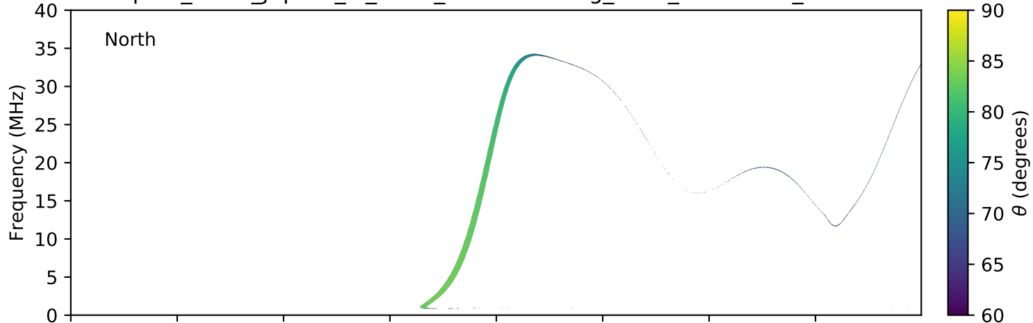
expres_earth_jupiter_io_isaac_lossc-wid1deg_3kev_20070413_v01.cdf
