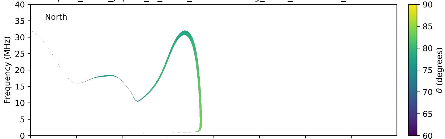
expres_earth_jupiter_io_isaac_lossc-wid1deg_3kev_20070412_v01.cdf
